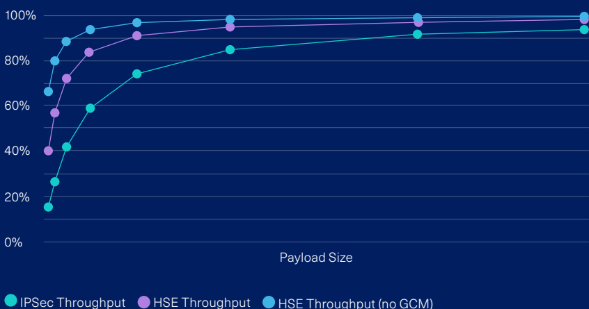
Figure 3. Available bandwidth per payload size (0-1400)
